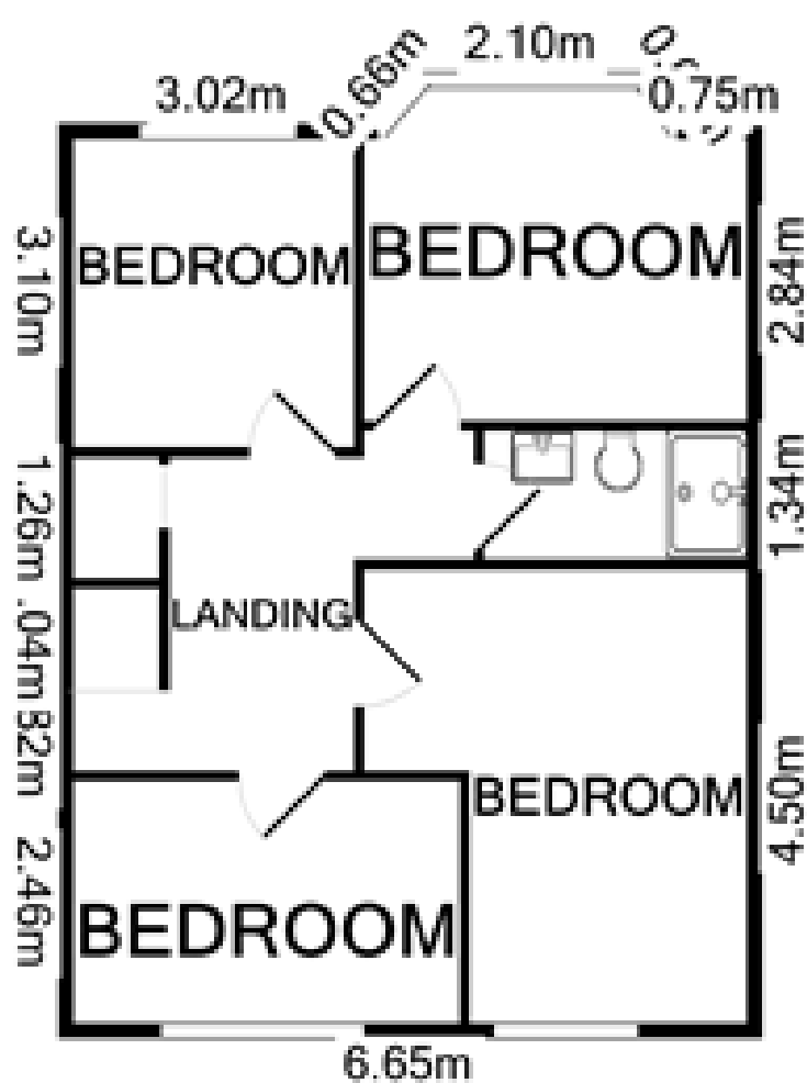
1ST FLOOR
